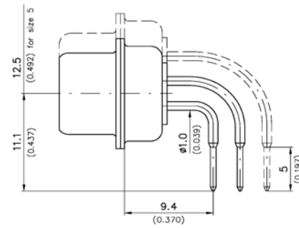
STYLE B Spacing 2.84mm (0.112") Pin Ø 0.6mm (0.024")
